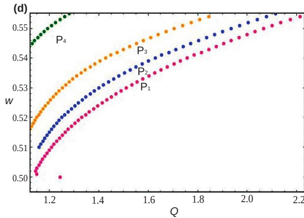
Fig. 4. The graph of wave vector Q vs frequency W (de-dimensionised parameters) for Different value of P where D1 = 0.5 and D2 = 0.5 .
