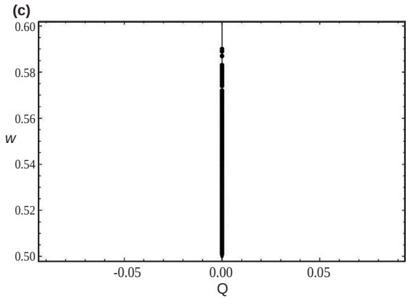
Fig. 3c. The graph of wave vector Q vs frequency W (de-dimensionlised parameters) for positive and negative Imaginary values where filling factor is constant.
