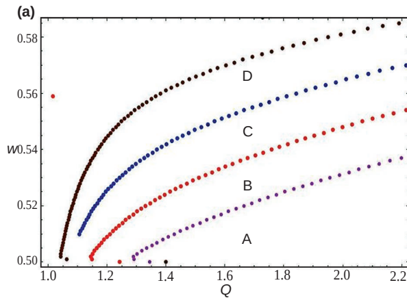
Fig. 3a. Plot of wave vector Q vs frequency W (de-dimensionlised parameters) for positive real values where filling factor is constant.
