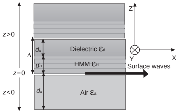
Fig. 1. An illustration of dielectric hyperbolic media with air at its surface, the photonic hyper crystal is terminated with air.
