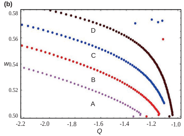
Fig. 3b. The graph of wave vector Q vs frequency W (de-dimensionlised parameters) for negative real values where filling factor is constant.
